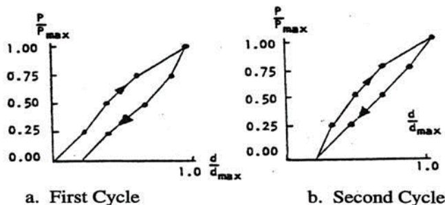
Figure 1. Static Load Test Load-Deflection Curves
